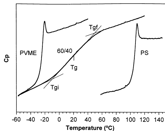
Figure 1. Differential scanning calorimetry traces of pure PS and PVME and of a 60/40 PS/PVME miscible blend. The C_p values (Y scale) have been adjusted to highlight width difference in the transition between the blend and the homopolymers. The initial and final T_g ( T_{gi} and T_{gf} ) were determined as shown.
