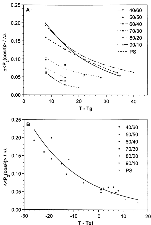
Figure 6. Slope of the deformation curves ( \Delta\langle P_2(\cos \theta) \rangle / \Delta\lambda ) as a function of the relative deformation temperature ( T - T_{\text{ref}} ) using (A) T_g as the reference temperature and (B) T_{gf} as the reference temperature.
